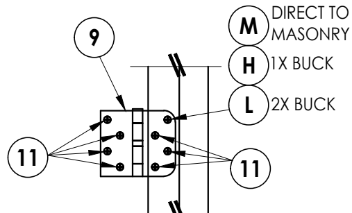
HINGE DETAIL
