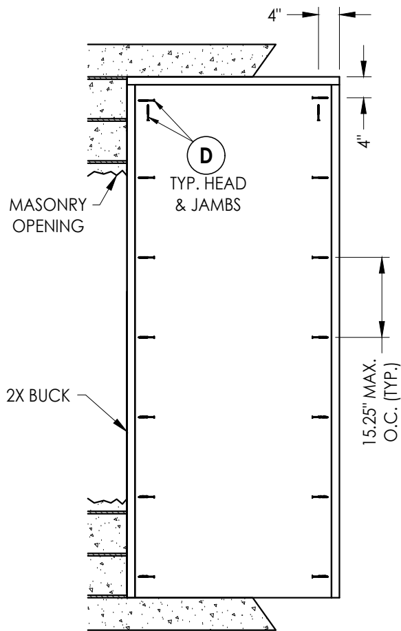
BUCK ANCHORING
