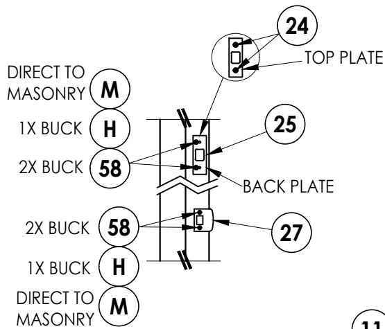
STRIKE DETAIL Schlage Hardware
