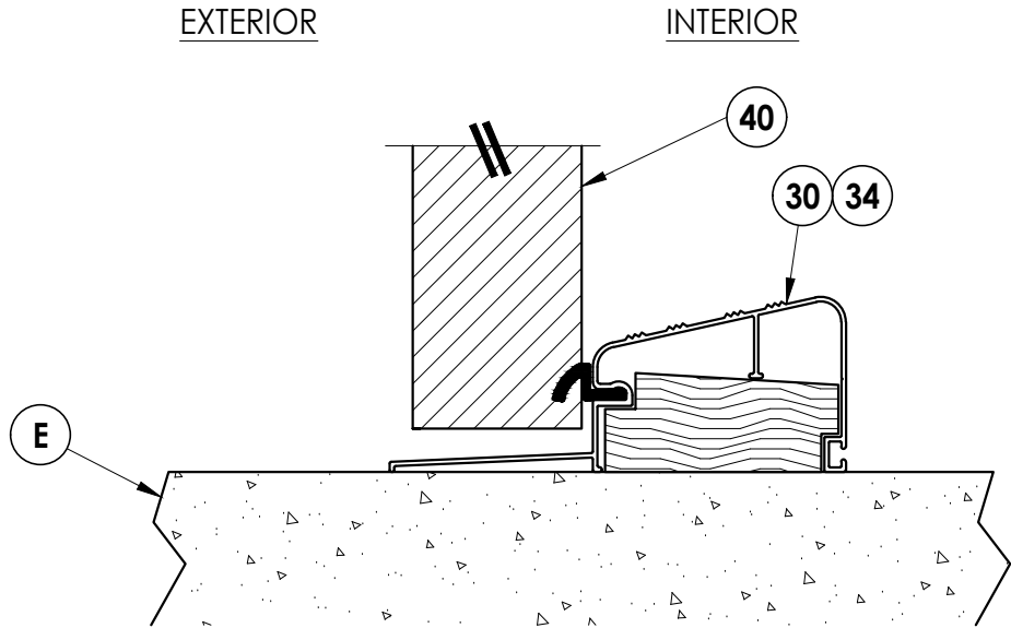
1 7 VERTICAL CROSS SECTION
