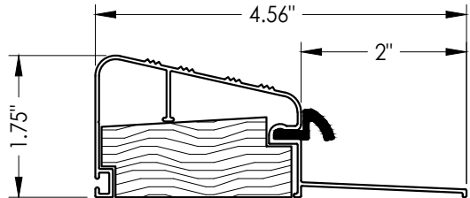
30 OUTSWING THRESHOLD DLP (QOSR)
