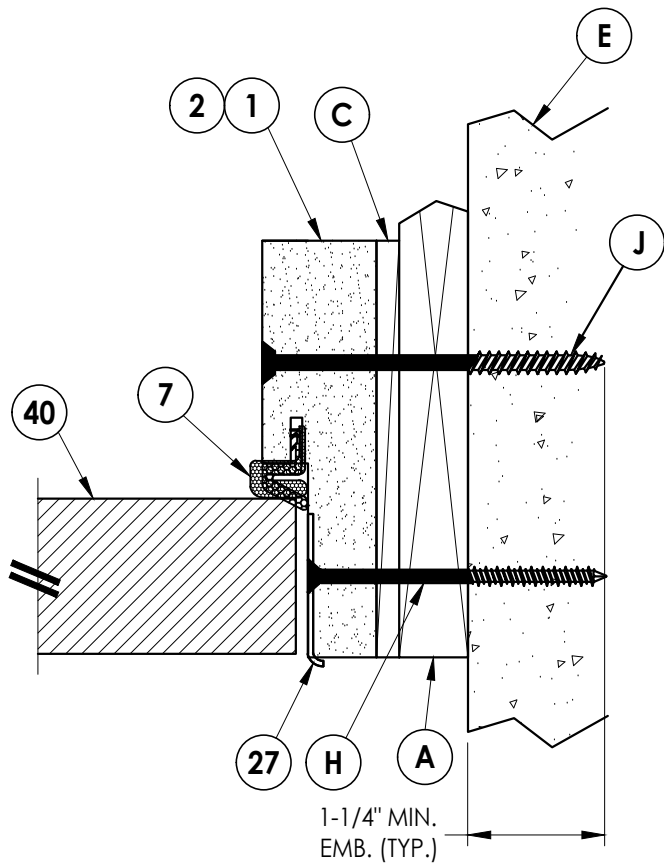
2 4 HORIZONTAL CROSS SECTION Shown w/ 1X sub-buck Outswing
