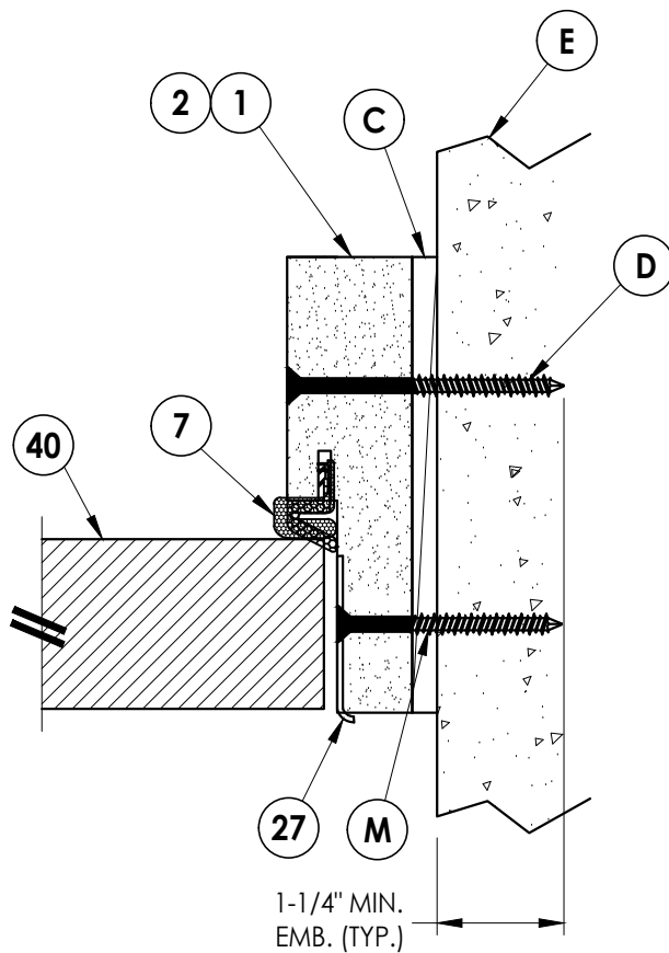
2 5 HORIZONTAL CROSS SECTION Shown Direct to Masonry Outswing
